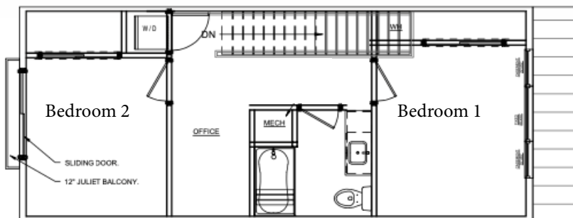
Second Floor - 575 SF
