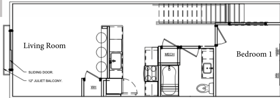
Second Floor - 678 SF
